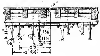
Fig. 297. Transverse Section.
